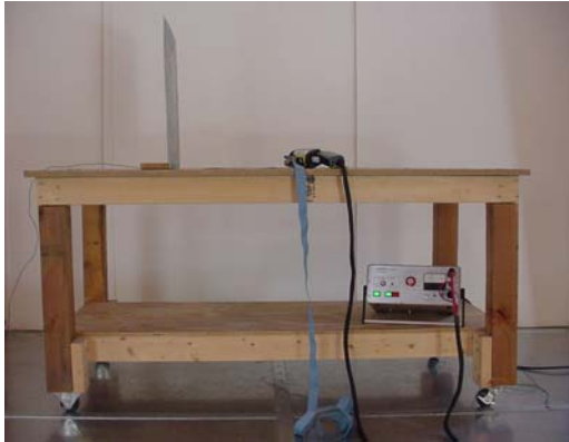
EN 61000-4-2 Electro-Static Discharge 8 kV Contact, 15 kV Air Discharge
